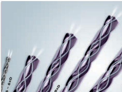
High performance twist drill/Micro twist drill solid carbide – PKD
